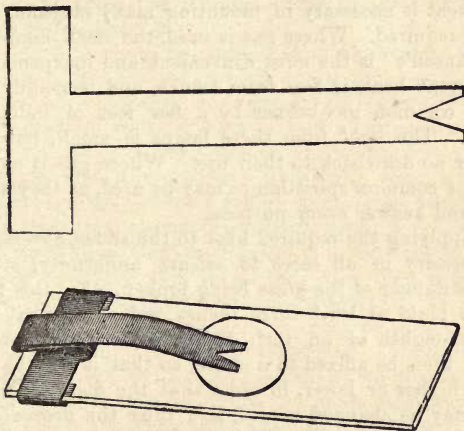
STEEL CLIP.
